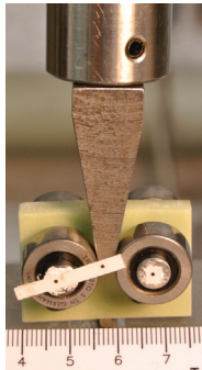
Wedge splitting test on bone cement
