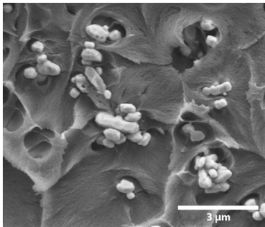
Fracture surface of bone cement
